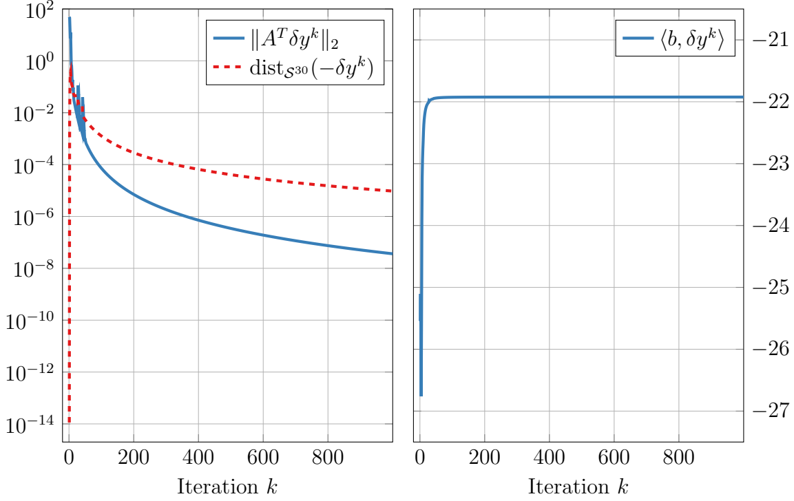
Figure 5: Convergence of \{\delta y^k\}_{k \in \mathbb{N}} to a certificate of primal infeasibility for problem infp1 from SDPLIB.
